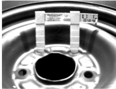
Figure 1 Model 45 is shown measuring a GM wheel with a 4 ¾" mounting pattern. The long legs allow easy reading of the bolt circle scales, which are directly displayed in the published manufactures sizes.
