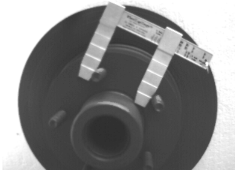
Figure 2 Model 45 is shown measuring a Ford front hub with a 4 ½" bolt circle. The reference marks on the legs assist taking the measurement if the hub gets in the way.
